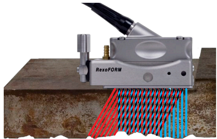
Example of beam possibilities with the RexoFORM and A14 probe.
