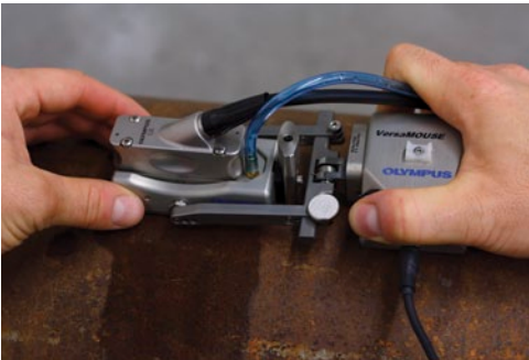
VersaMOUSE scanner and RexoFORM for corrosion inspection.
